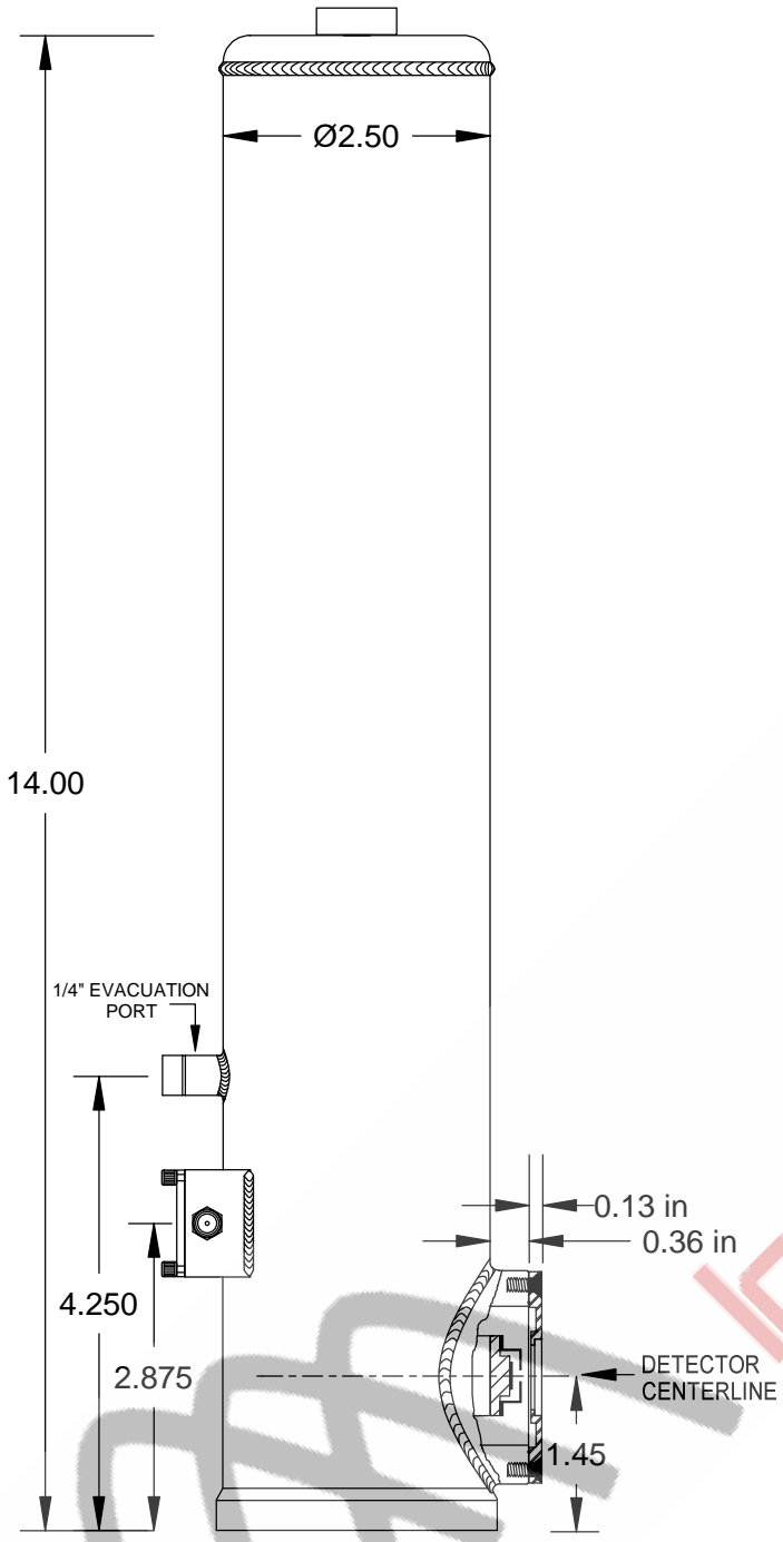
SIDE VIEW MSL-24
