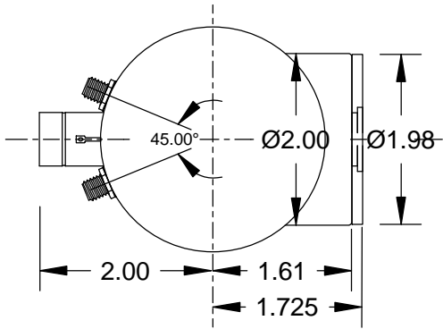
SIDE VIEW MSL-8
