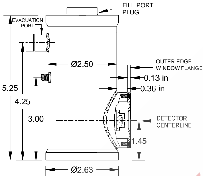
SIDE VIEW MSL-8
