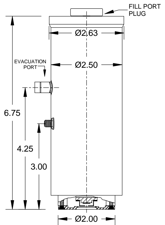
SIDE VIEW MDL-12
