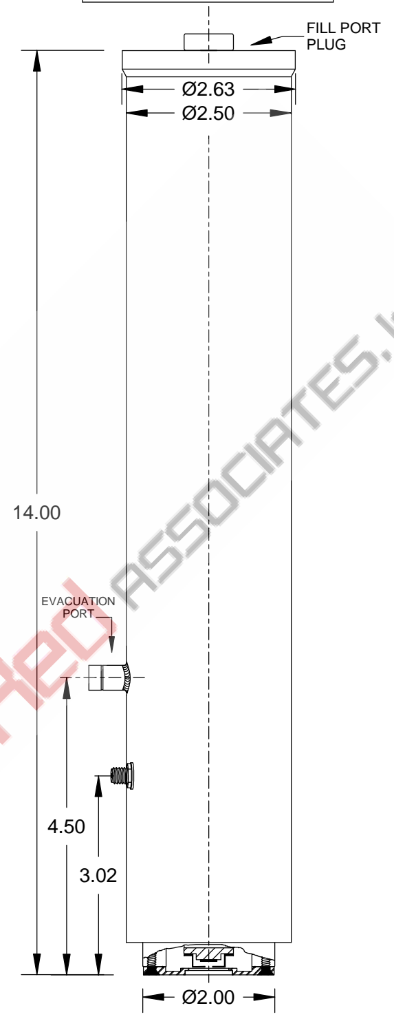
SIDE VIEW MDL-24
