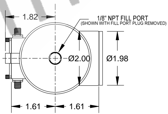
TOP VIEW MSL-24
