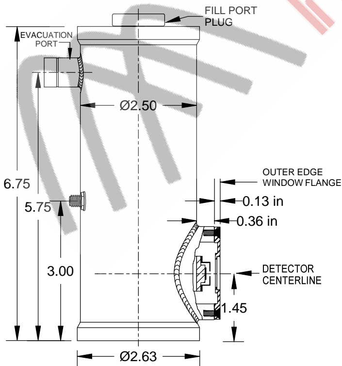
SIDE VIEW MSL-12
